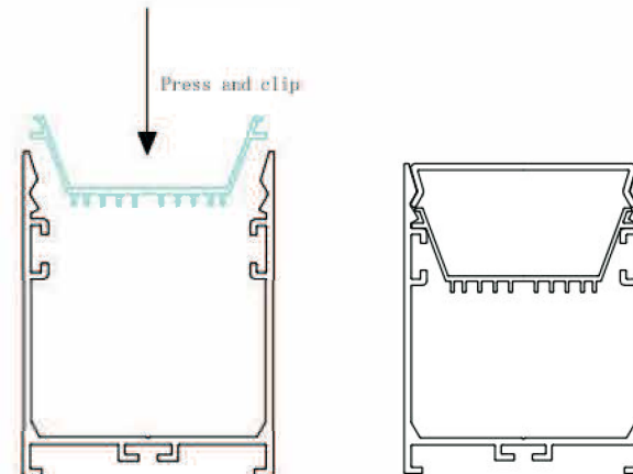
TG-S5470 assembly:
